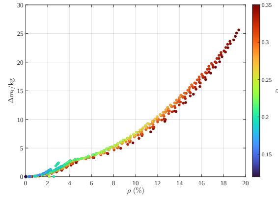
Fig. 12. Relationship between the non-low-thrust mode fraction \rho and mass gain \Delta m_f .
