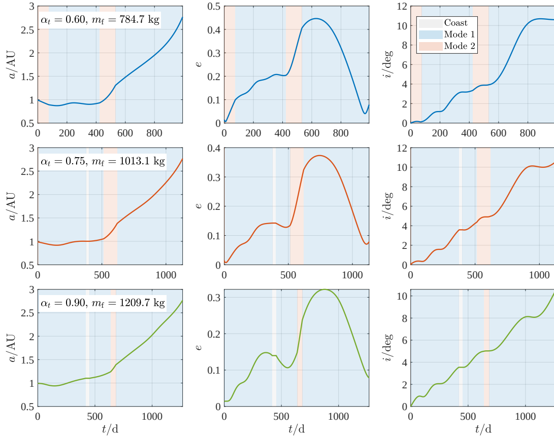
Fig. 5a. Variations of semimajor axis, eccentricity, and inclination with mode-activity shading.
