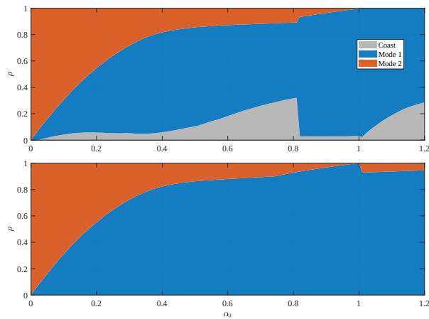
Fig. 9. Mode-time fractions of the dual-mode schemes as \alpha_f varies.
